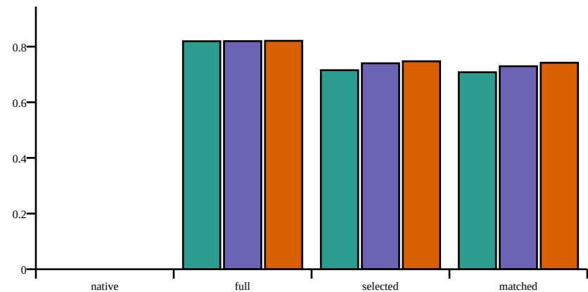
Max-3SAT: auxiliary inconsistency
