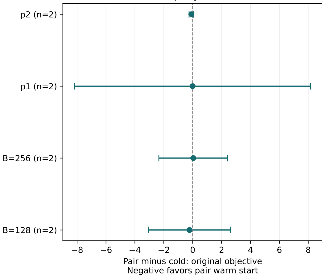
Spin glass
