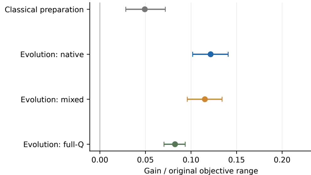
Weighted Max-3SAT (30 independent instances)
