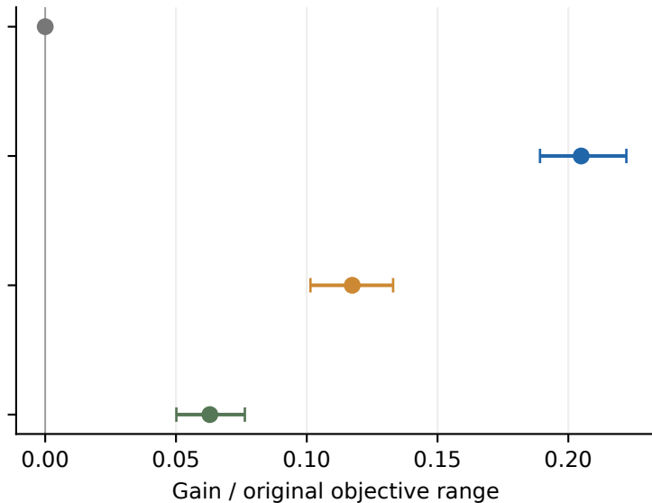
Cubic spin glass (30 independent instances)
