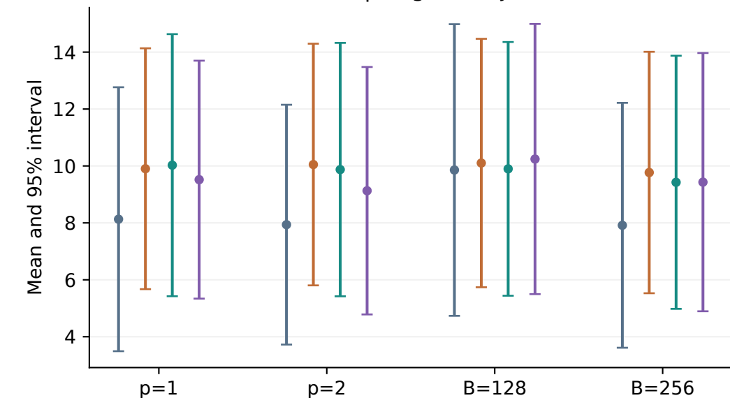
Max-3SAT | Original objective
