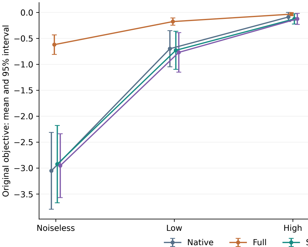
Cubic spin glass | n=9
