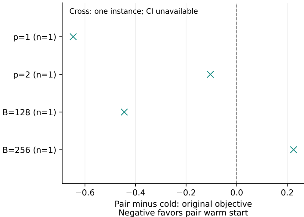
Cubic spin glass
