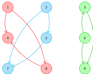
Figure: \mathcal{G}_D
