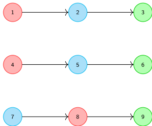
Figure: \mathcal{G}_C
