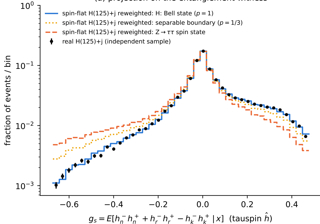
(a) projection on the entanglement witness
