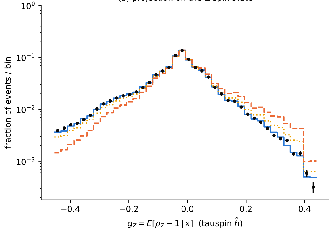
(b) projection on the Z spin state
