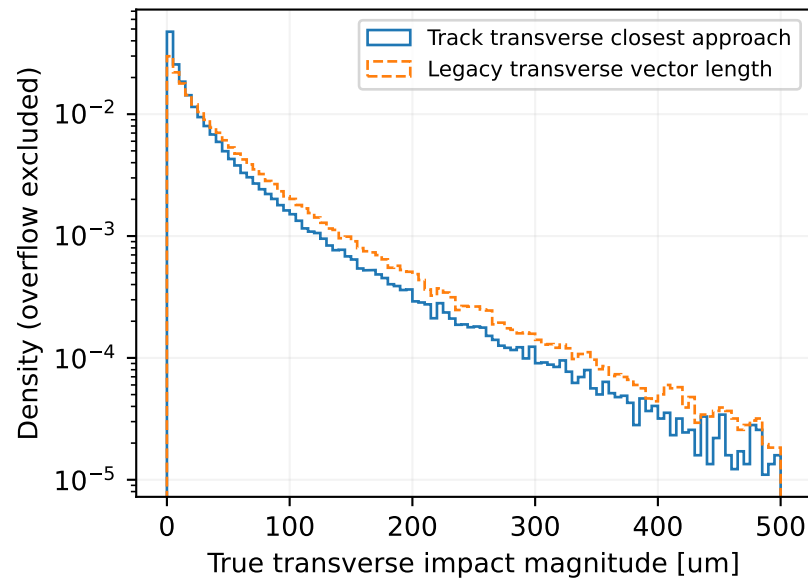
Toy lep-had MC before downstream selection: impact geometry and null resolution
