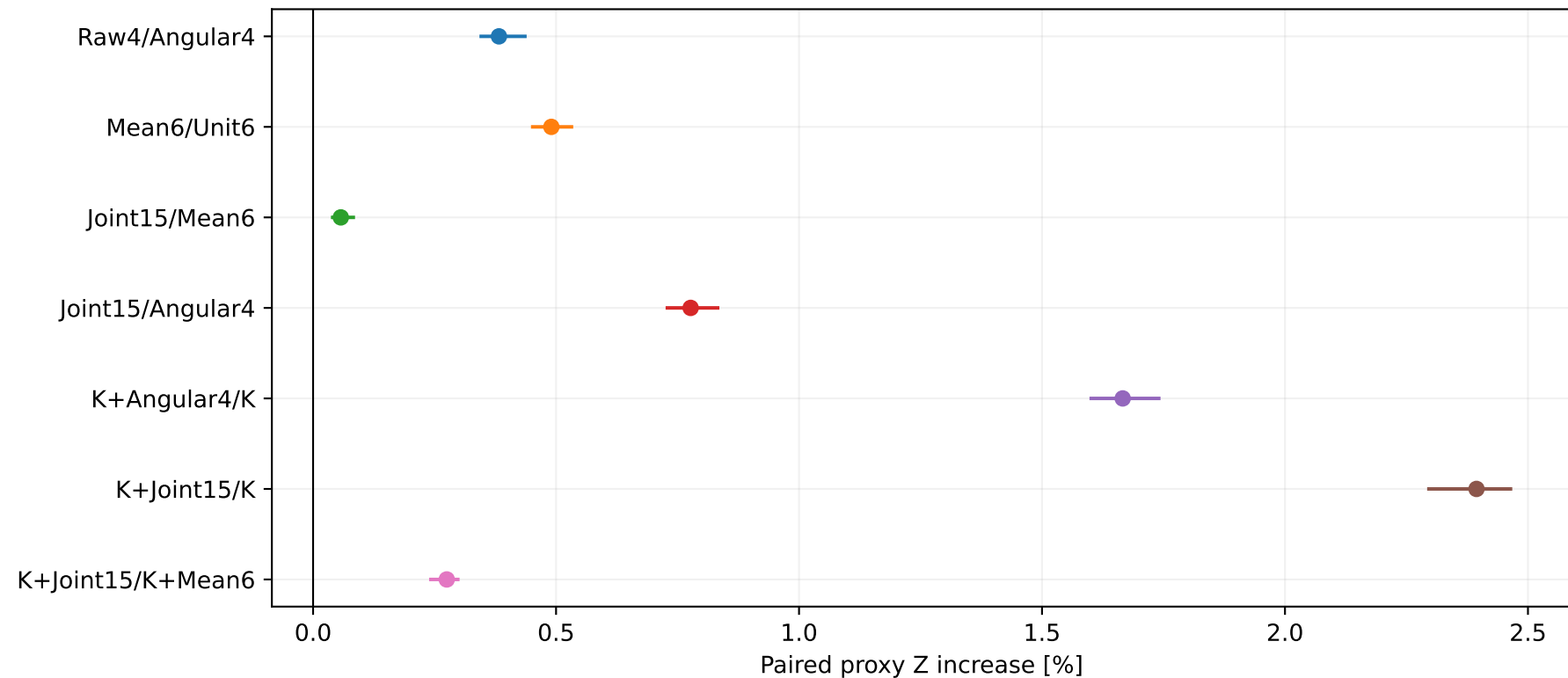
Seed 0, mHH > 350 GeV: 100 paired event bootstraps 68% MC intervals; classifiers and validation bins fixed
