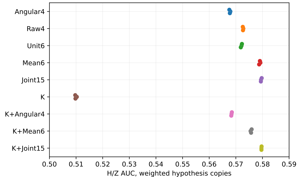
Same HH kinematics, m_{HH} > 350 GeV; three initializations per readout Fixed illustrative S=40 , B=160 ; H/Z/W/U mixture; normalization and contrast profiling
