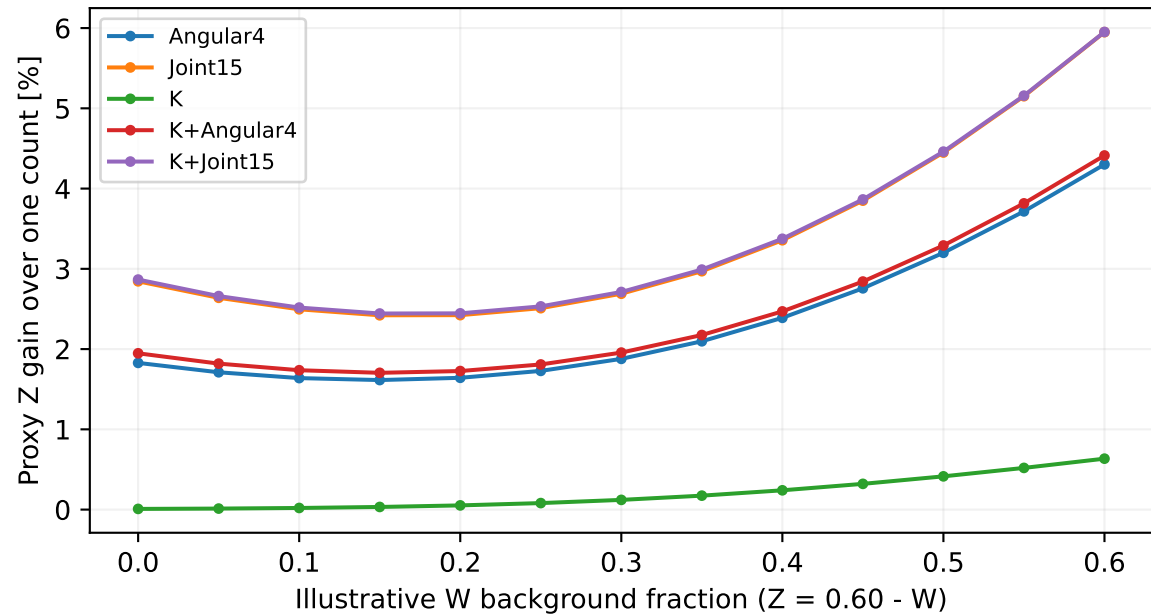
Conditional spin experiment: no production-kinematic H/Z separation Single H=0.28 and U=0.12 fixed; no ATLAS background-fraction inference
