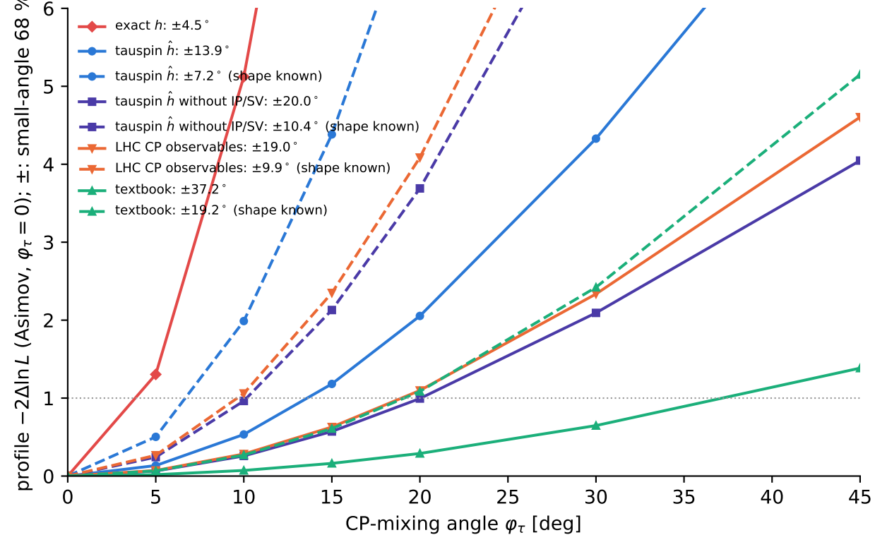
(b) tau Yukawa CP angle, \tau_h \tau_h only, 3 \text{ ab}^{-1} , one experiment
