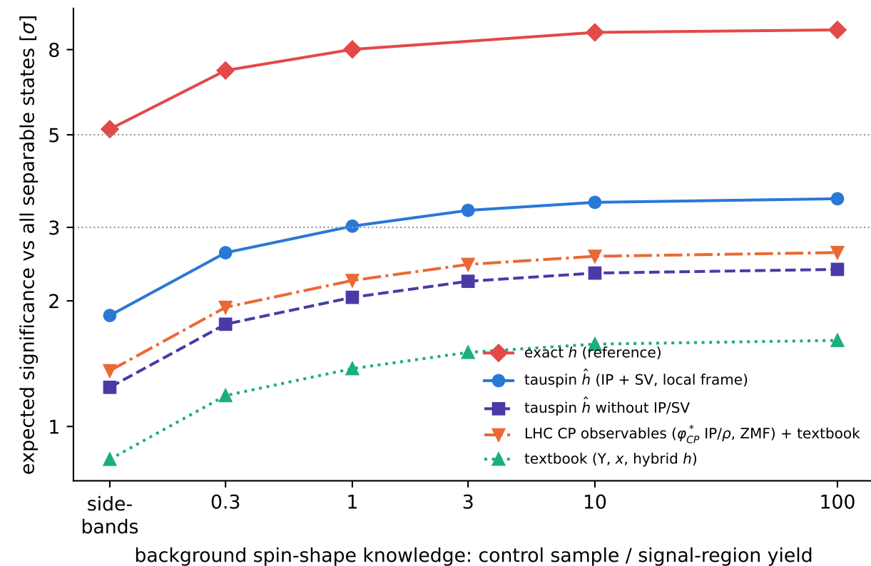
(a) spin entanglement in H \rightarrow \tau_h \tau_h , 3 \text{ ab}^{-1} , one experiment
