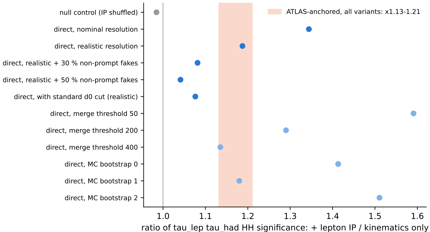
(a) lepton lifetime information in tau_lep tau_had ( 3 \text{ ab}^{-1} )
