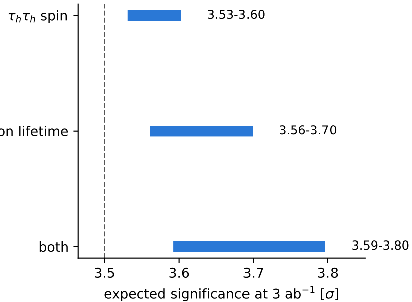
ATLAS b\bar{b}\tau\tau (published 3.5)
