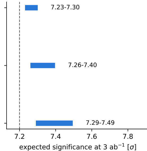
ATLAS+CMS HH (published 7.2)
