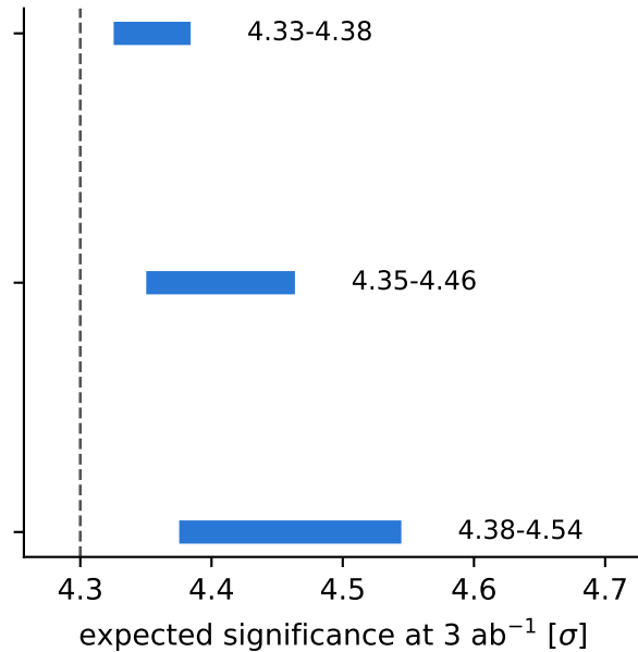
ATLAS HH combination (published 4.3)
