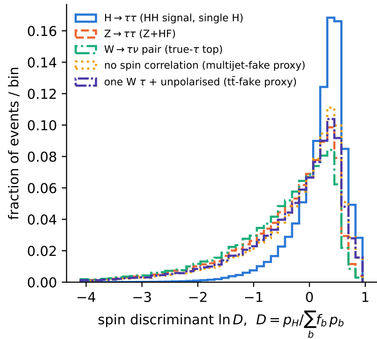
exact h (truth)
