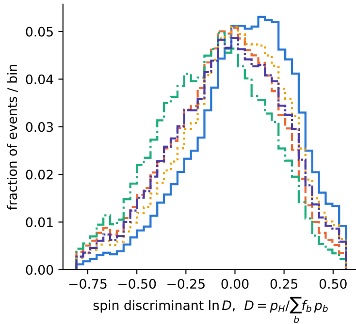
reco h_{\text{pred}} (3 IP + SV, ATLAS full sim)
