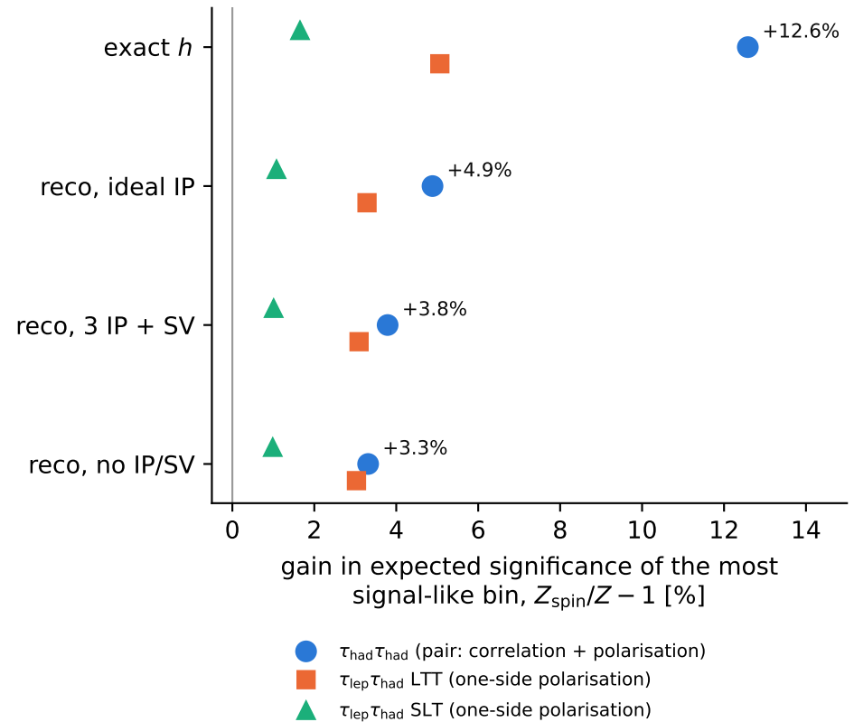
spin binning added to the ATLAS Run-2 top bin ( 3 \text{ ab}^{-1} )
