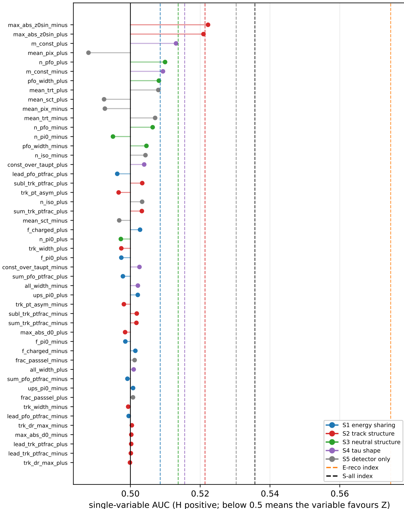
Substructure variables one at a time, and the cross-fitted block indices held-out report subset, 44,887 events
