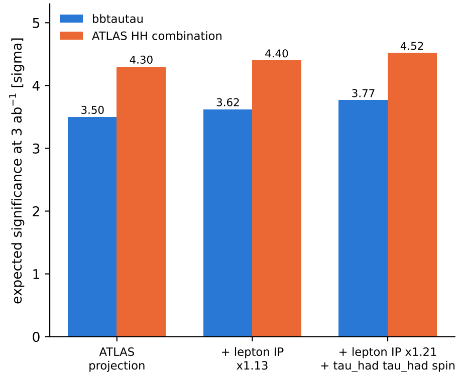
(b) illustrative transfer (ratios applied to ATL-PHYS-PUB-2024-016)
