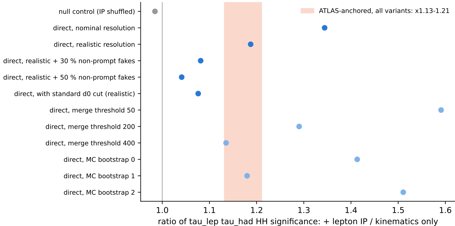
(a) lepton lifetime information in tau_lep tau_had ( 3\text{ ab}^{-1} )
