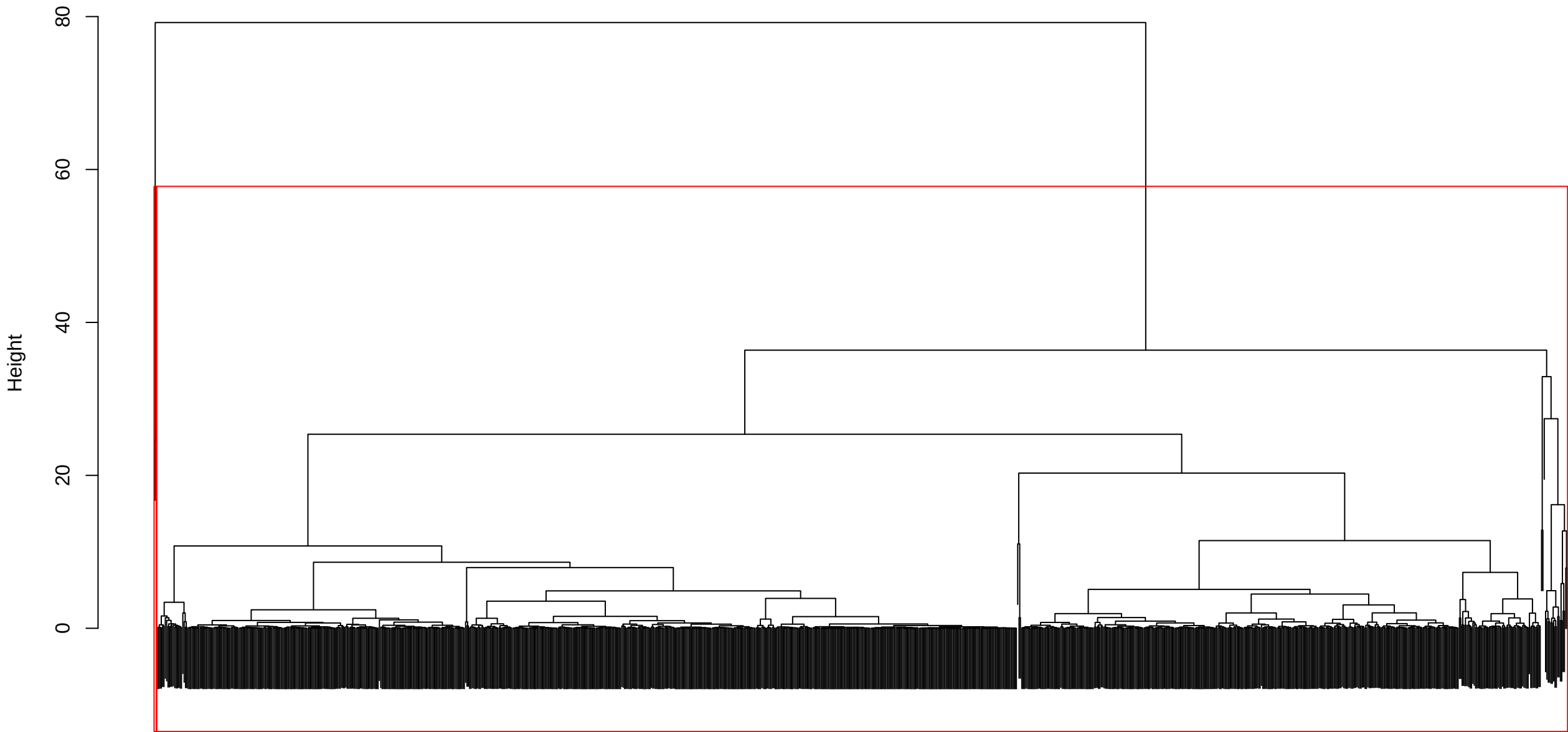
Dendrograma – Ward's Method (Sem Big 5)
