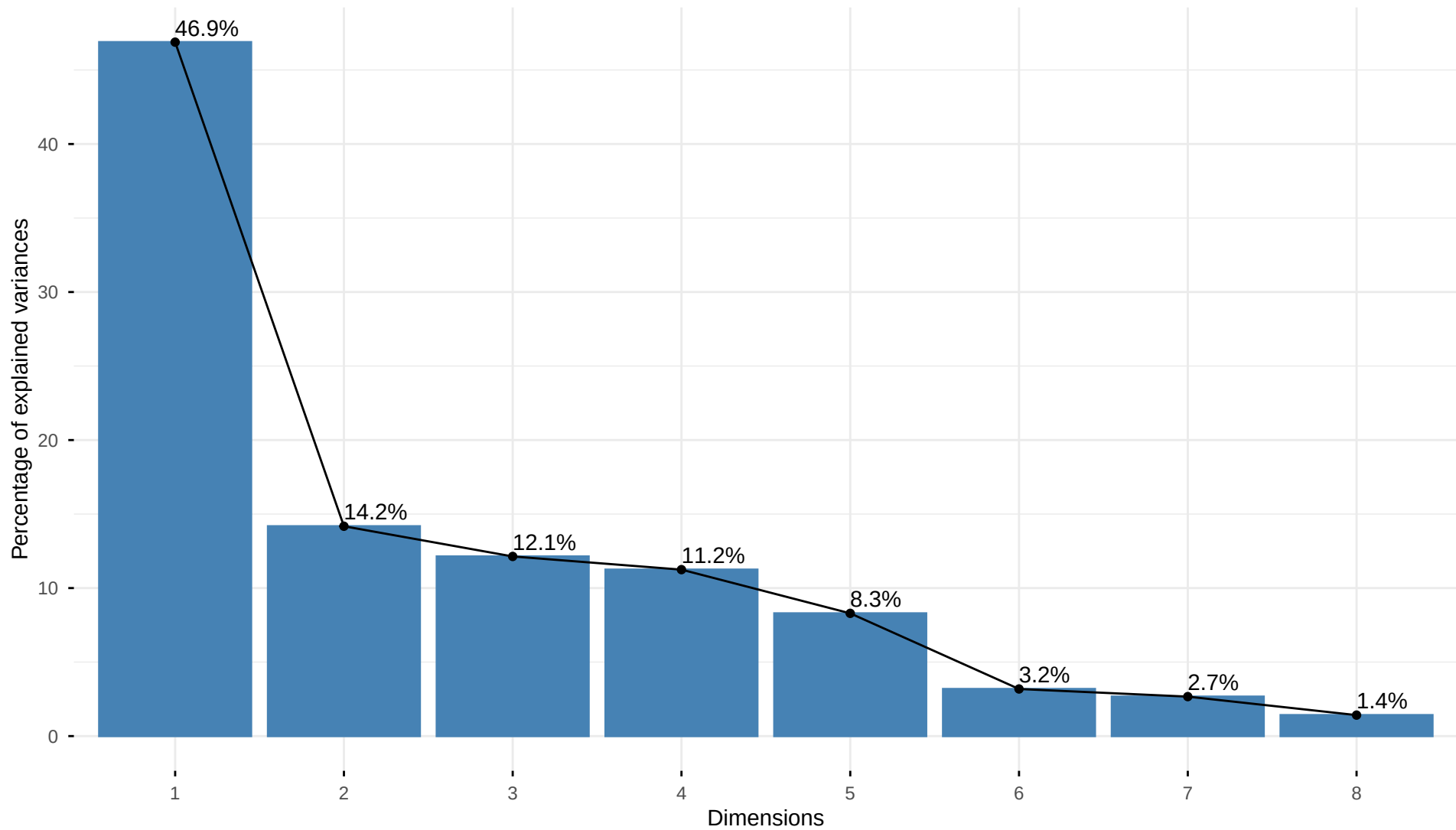
Scree Plot – PCA sem Big 7 (N=1,048)
