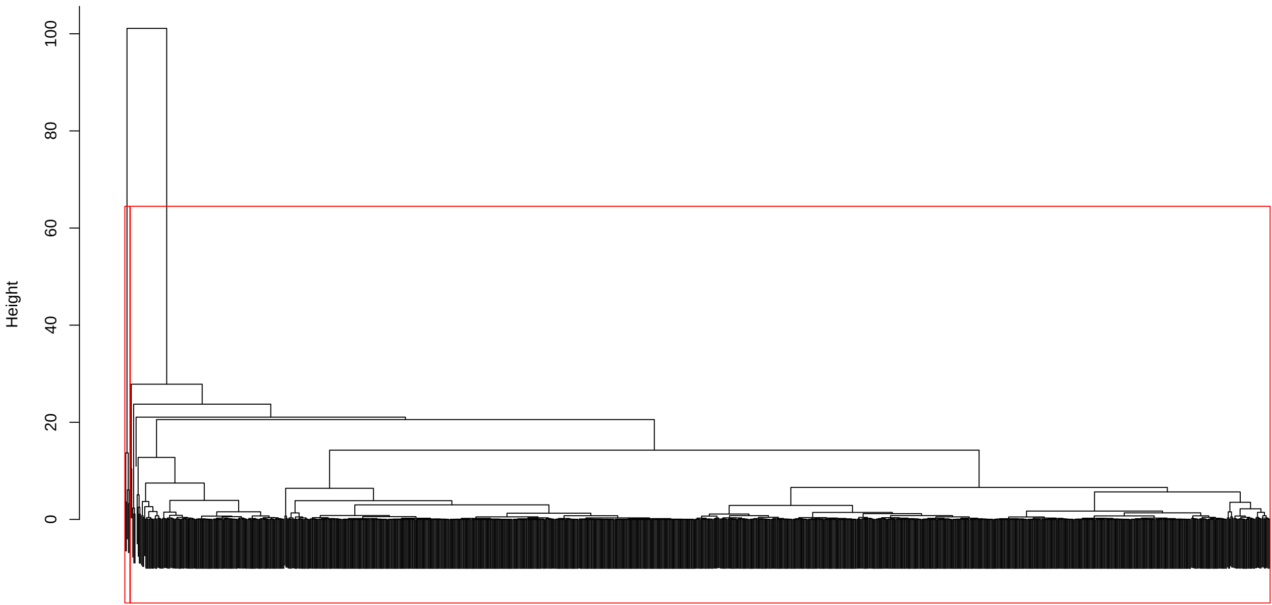
Dendrograma – Ward's Method
