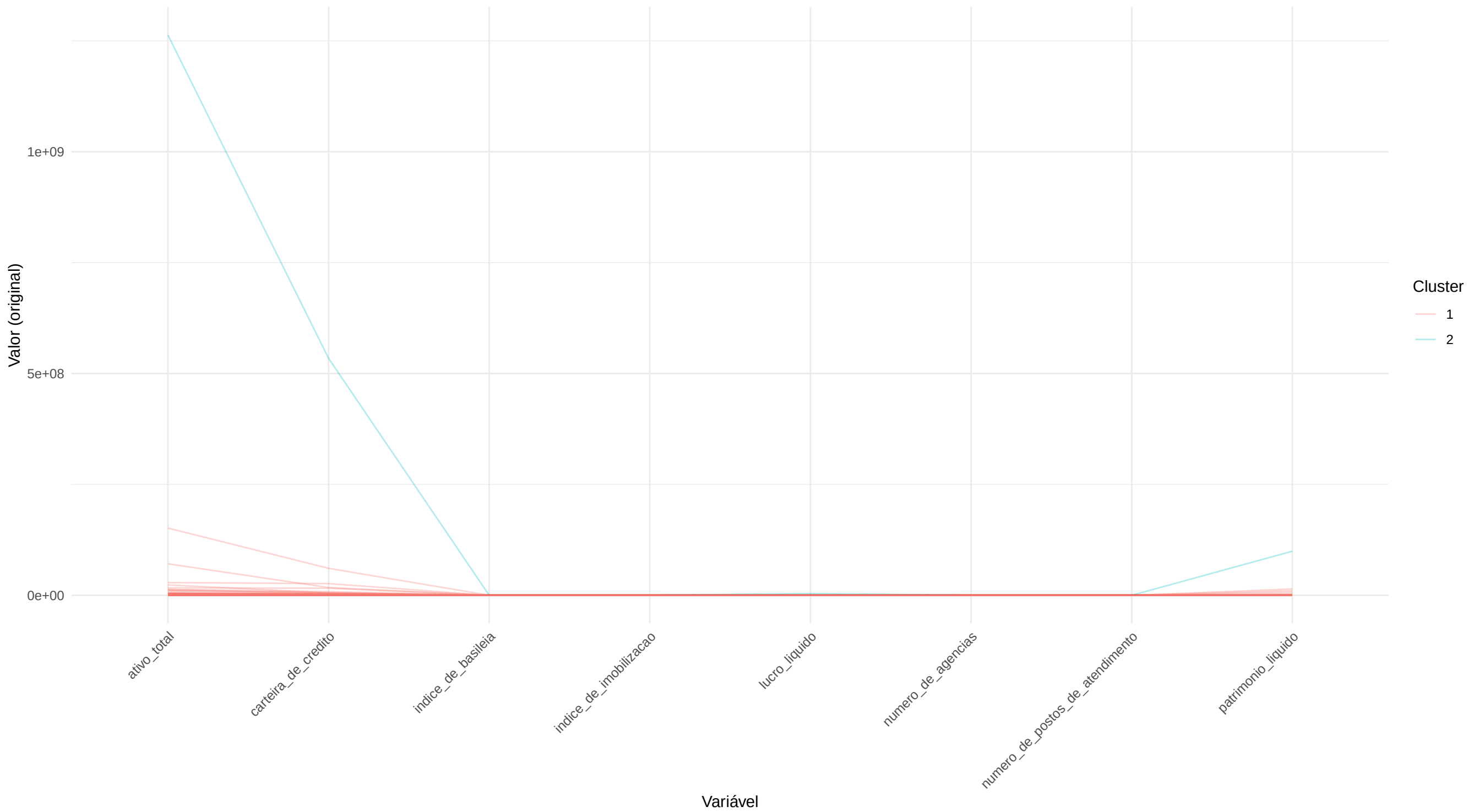
Parallel Coordinates – Perfis dos Clusters
