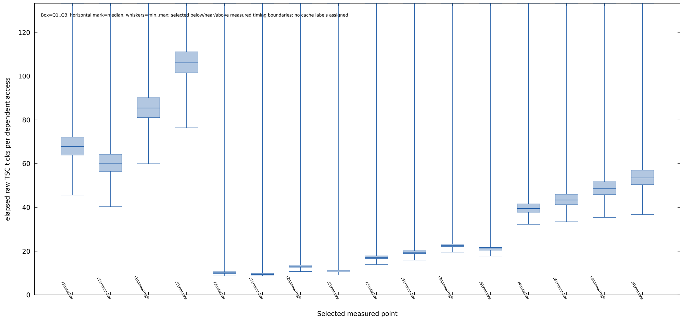
Q1-Q3 with min/max whiskers crux.ece.ncsu.edu latency representatives (x86 64 , TSC ticks)
