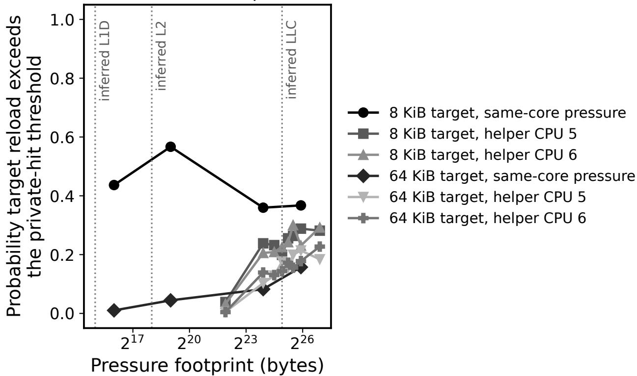
crux: cross-level eviction of a private-resident line
