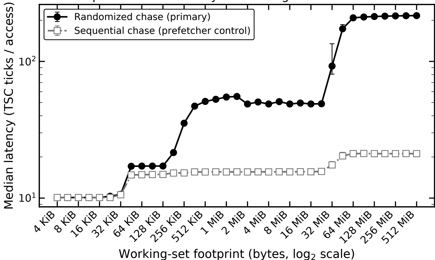
Dependent-load latency vs. working-set size -- sunbird
