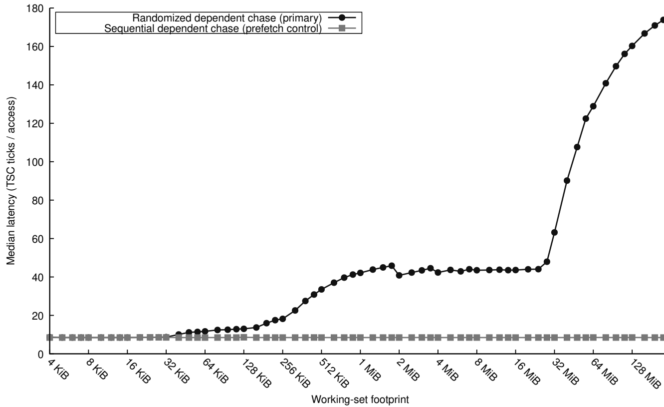
c202n08 Phase I prefetcher sanity control
