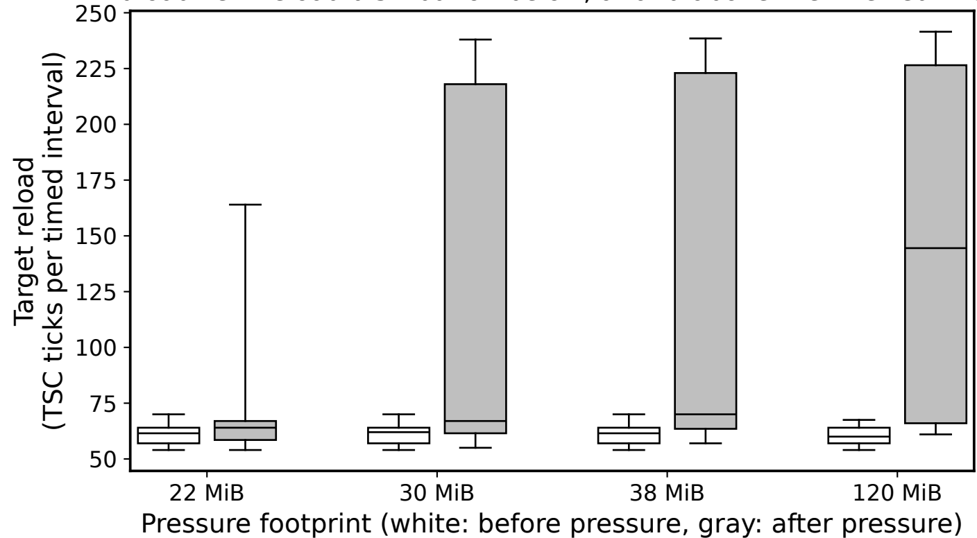
broadwell: reload distribution below, at and above the inferred LLC
