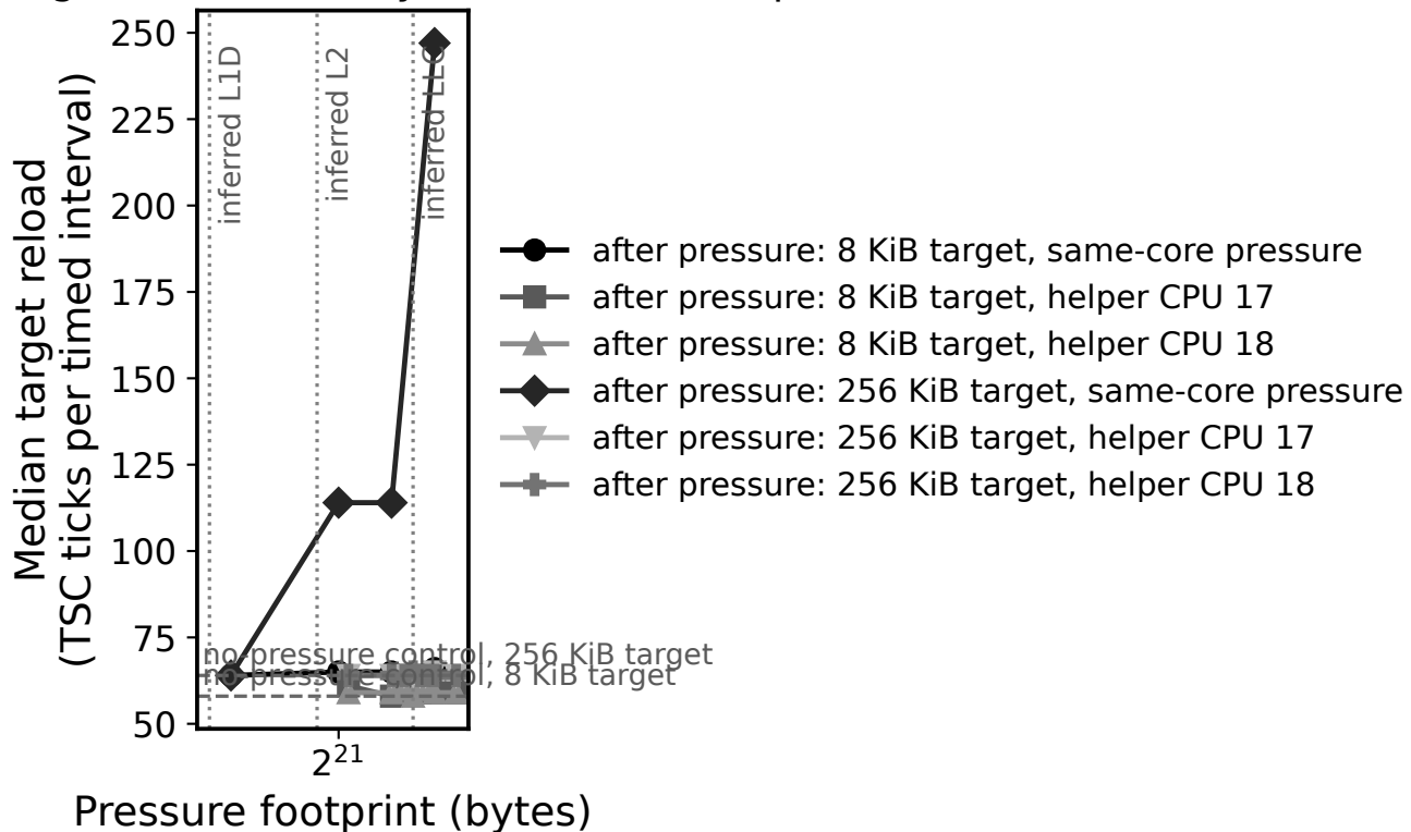
cascadelake: target reload latency after cross-level pressure
