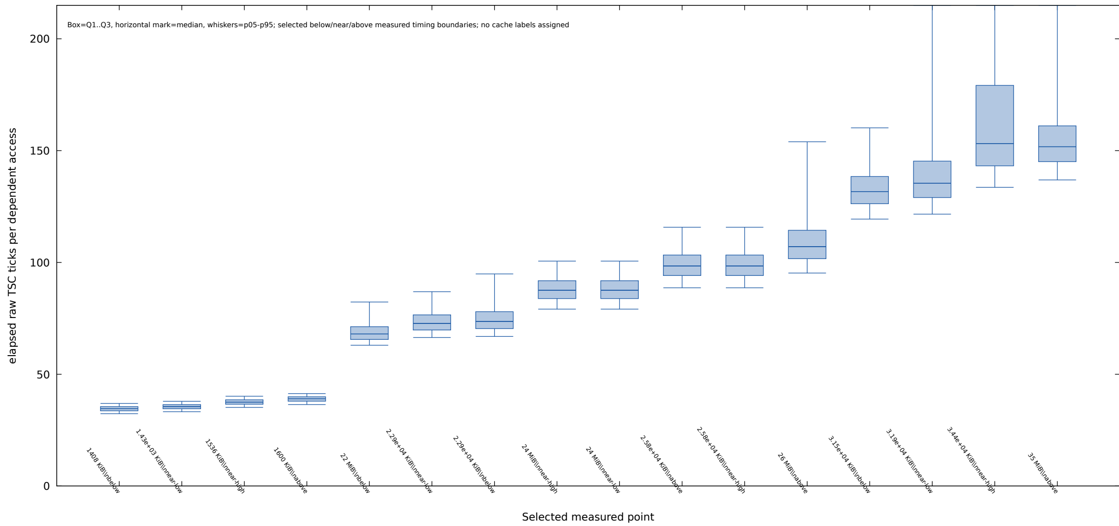
Q1-Q3 with p05-p95 whiskers c020n01 latency representatives (x86 64 , TSC ticks)
