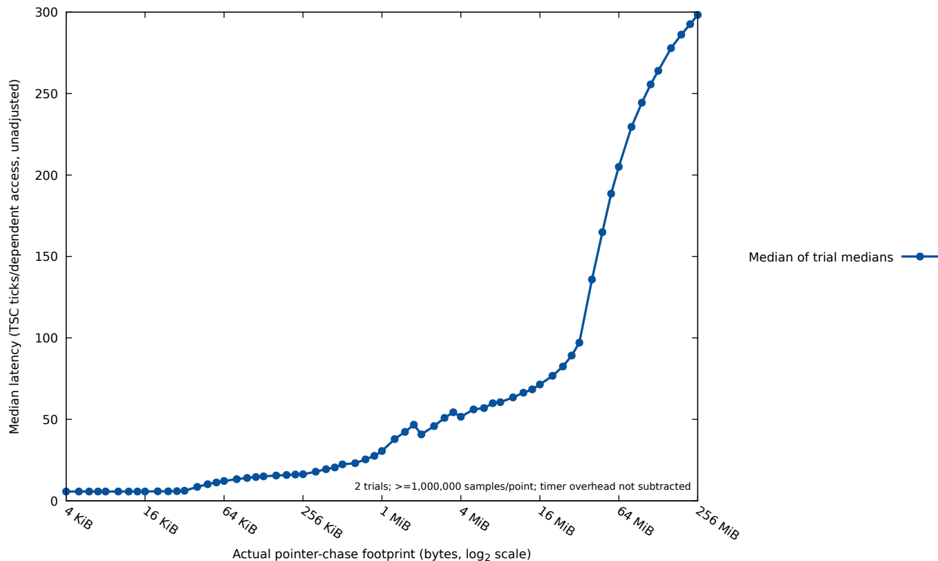
n0398 Phase I randomized dependent capacity sweep
