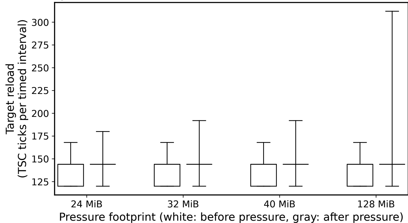
genoa: reload distribution below, at and above the inferred LLC
