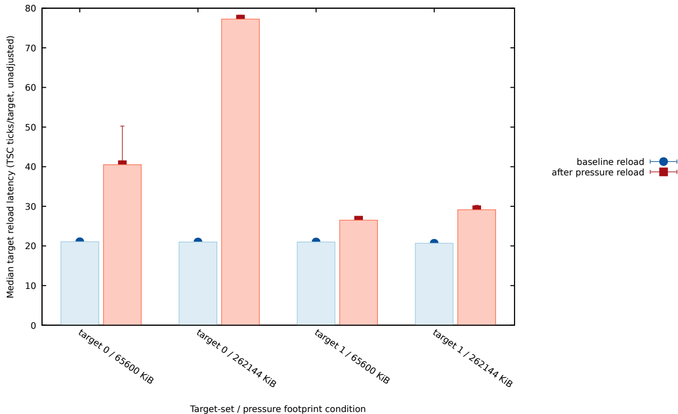
haswell e victiong30106 Phase I cross-level eviction/reload evidence
