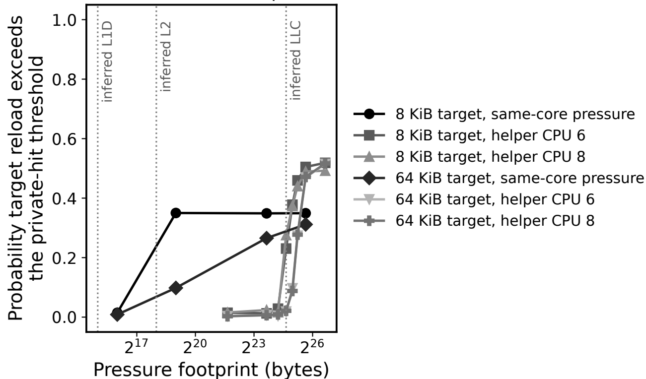
haswell: cross-level eviction of a private-resident line
