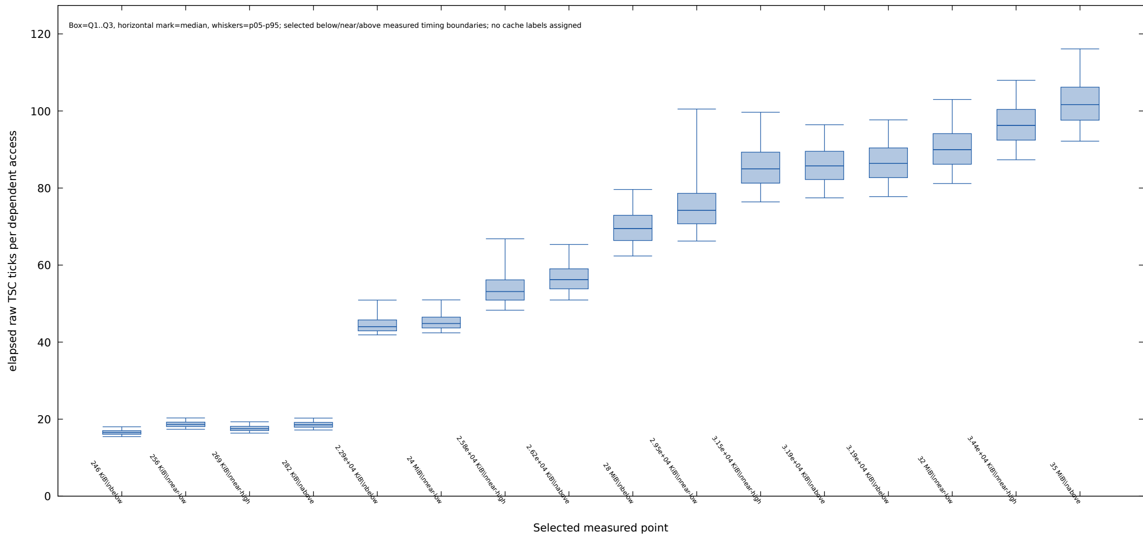
Q1-Q3 with p05-p95 whiskers c207n02 latency representatives (x86 64 , TSC ticks)
