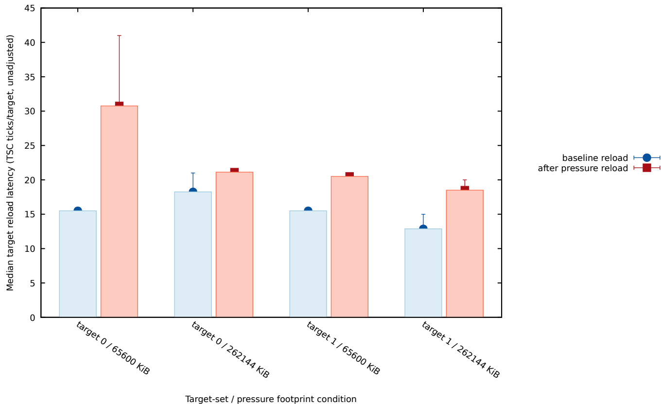
skylake e viction 832714 Phase I cross-level eviction/reload evidence
