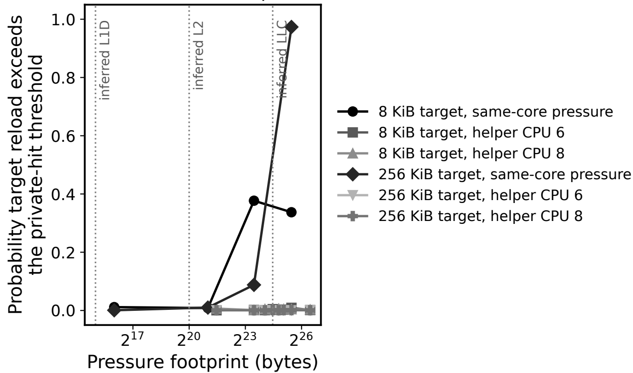
skylake: cross-level eviction of a private-resident line
