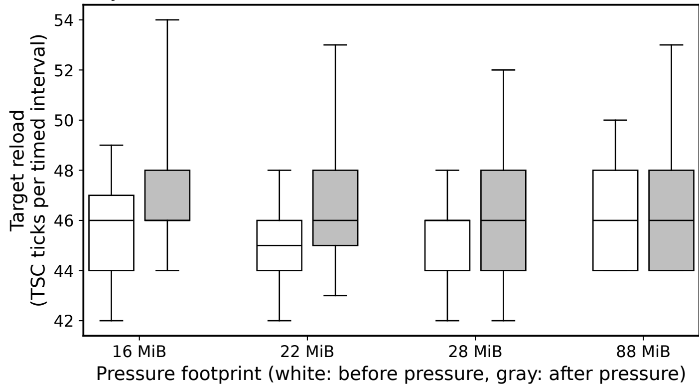
skylake: reload distribution below, at and above the inferred LLC
