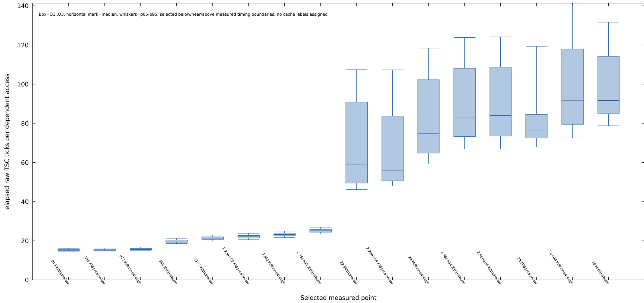
Q1-Q3 with p05-p95 whiskers c052n01 latency representatives (x86 64 , TSC ticks)
