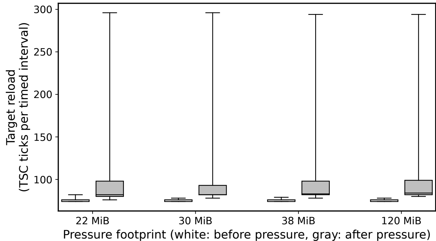
charnwood: reload distribution below, at and above the inferred LLC
