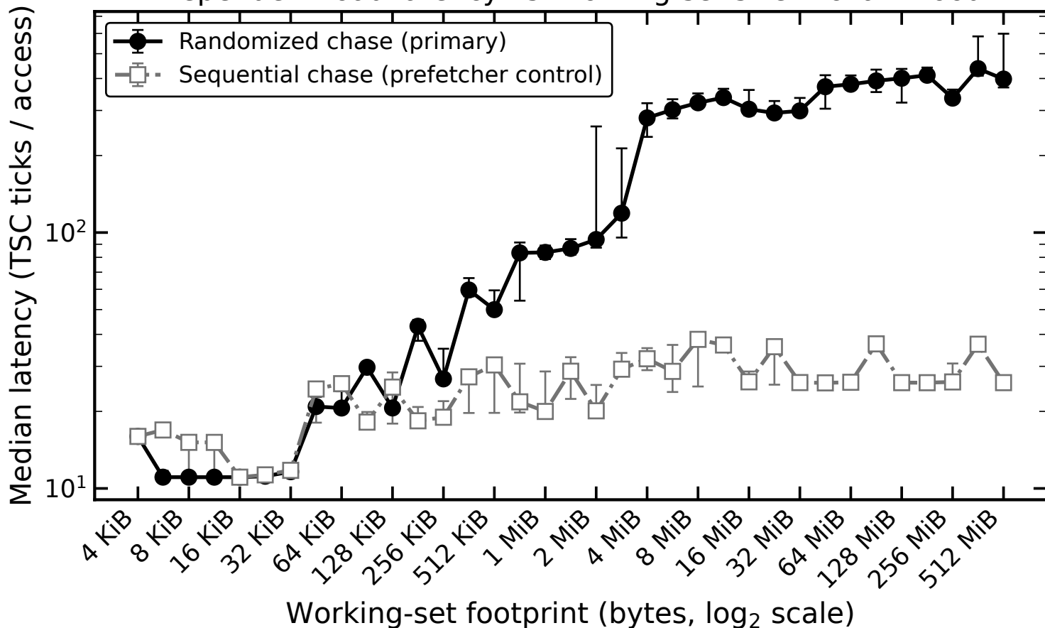
Dependent-load latency vs. working-set size -- charnwood
