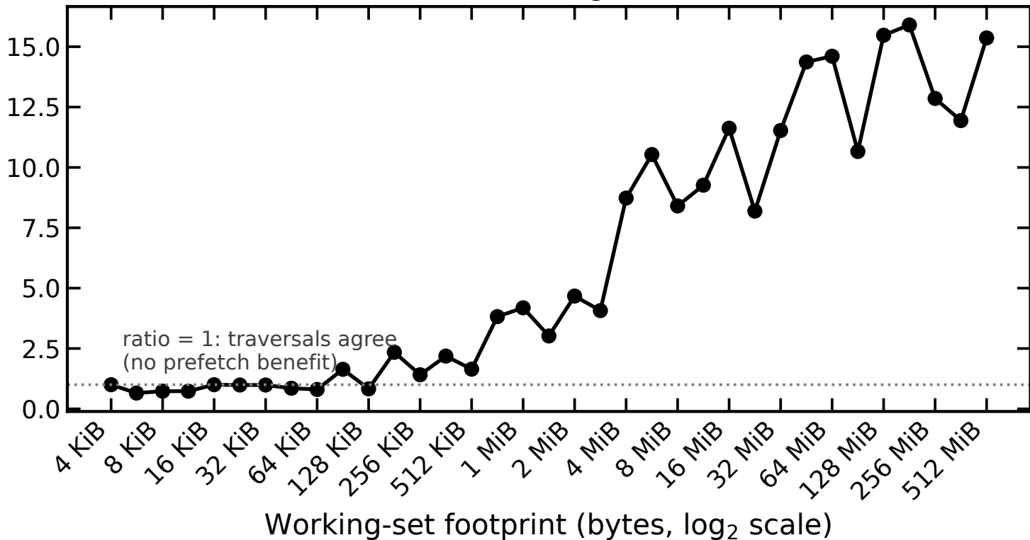
Prefetcher benefit vs. working-set size -- charnwood
