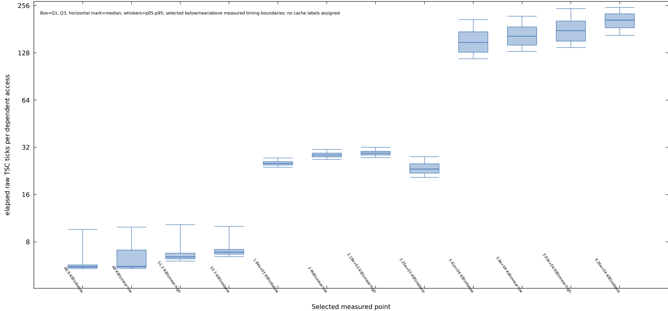
Q1-Q3 with p05-p95 whiskers artemisia.ece.ncsu.edu latency representatives (x86 64 , TSC ticks)
