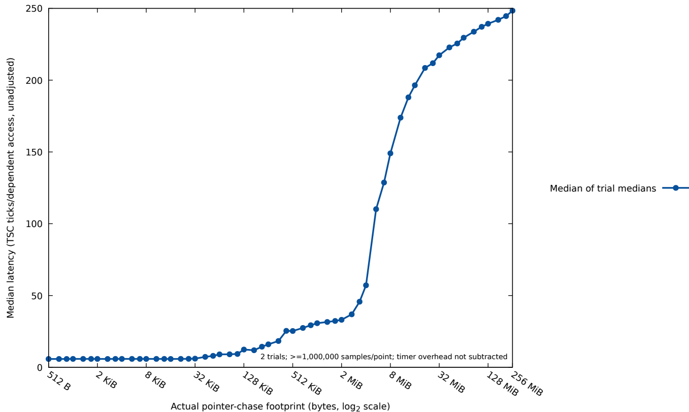
crux.ece.ncsu.edu Phase I randomized dependent capacity sweep
