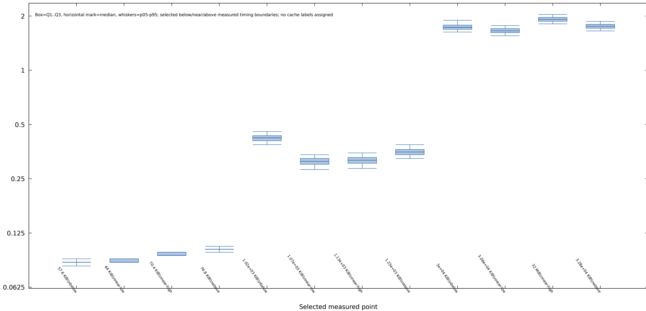
Q1-Q3 with p05-p95 whiskers thunderbird.ece.ncsu.edu latency representatives (aarch64, generic-timer ticks)
