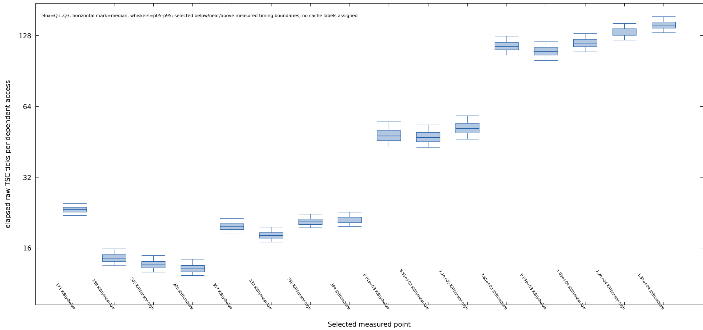
Q1-Q3 with p05-p95 whiskers upgrade.ece.ncsu.edu latency representatives (x86 64 , TSC ticks)
