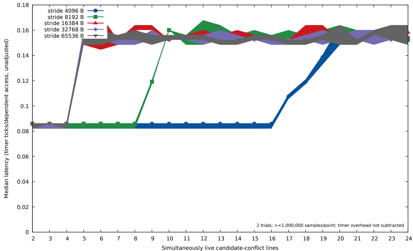
thunderbird.ece.ncsu.edu Phase I randomized conflict-set sweep
