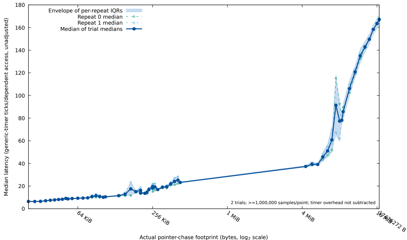
upgrade.ece.ncsu.edu Phase I randomized dependent capacity sweep
