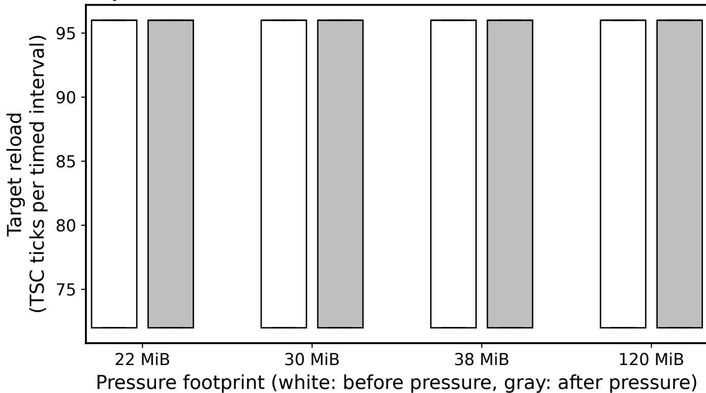
skylark: reload distribution below, at and above the inferred LLC
