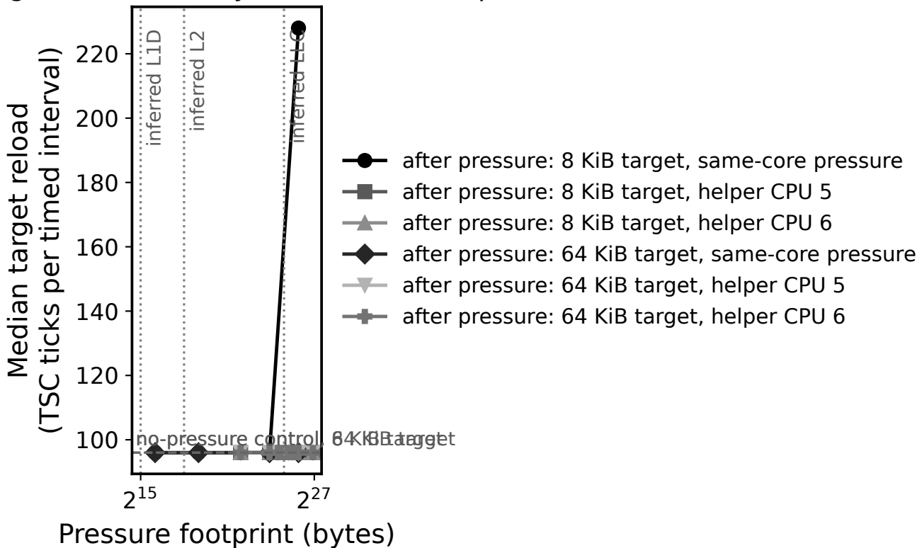
skylark: target reload latency after cross-level pressure
