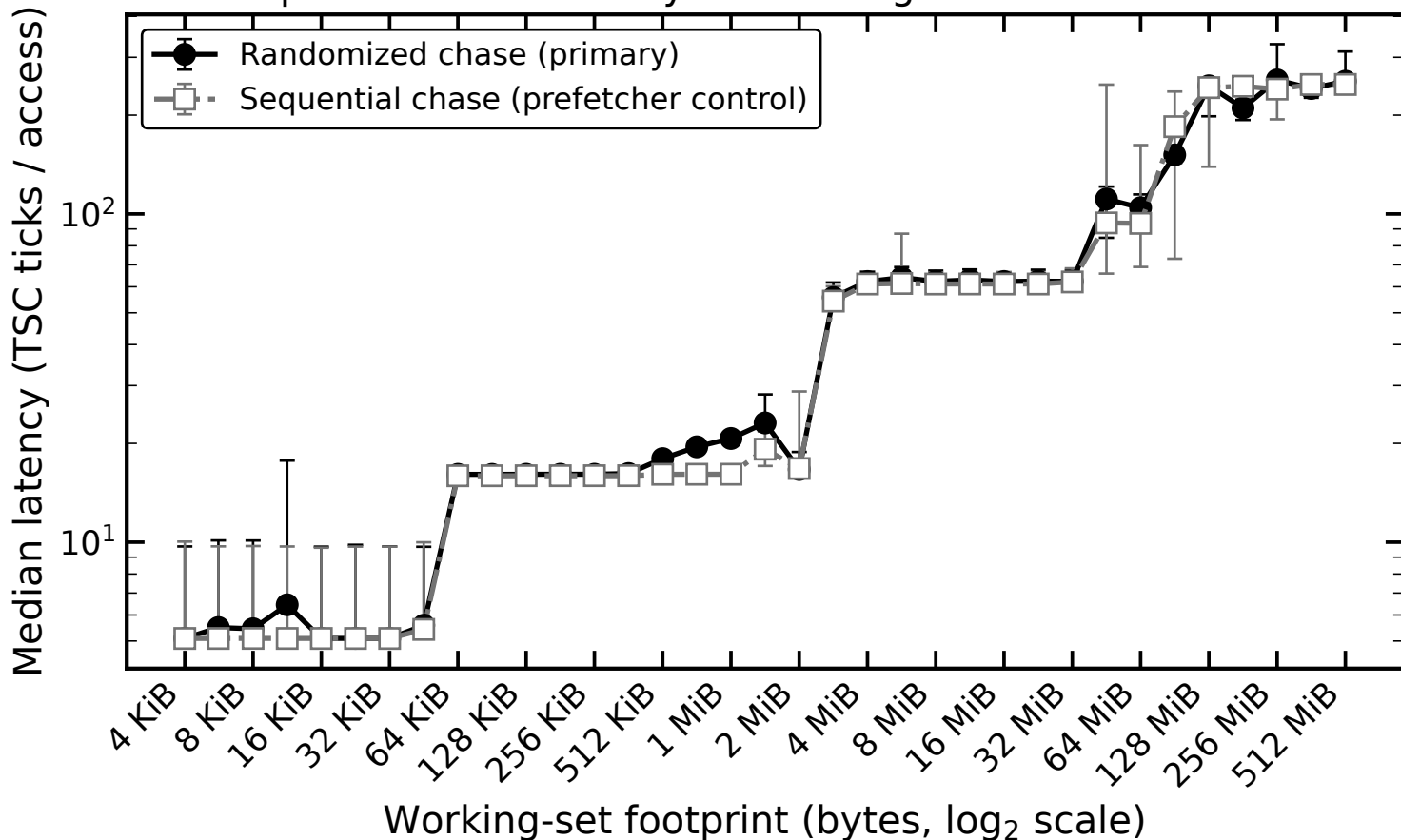
Dependent-load latency vs. working-set size -- artemisia
